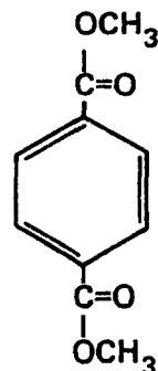
Dimethyl terephthalate
