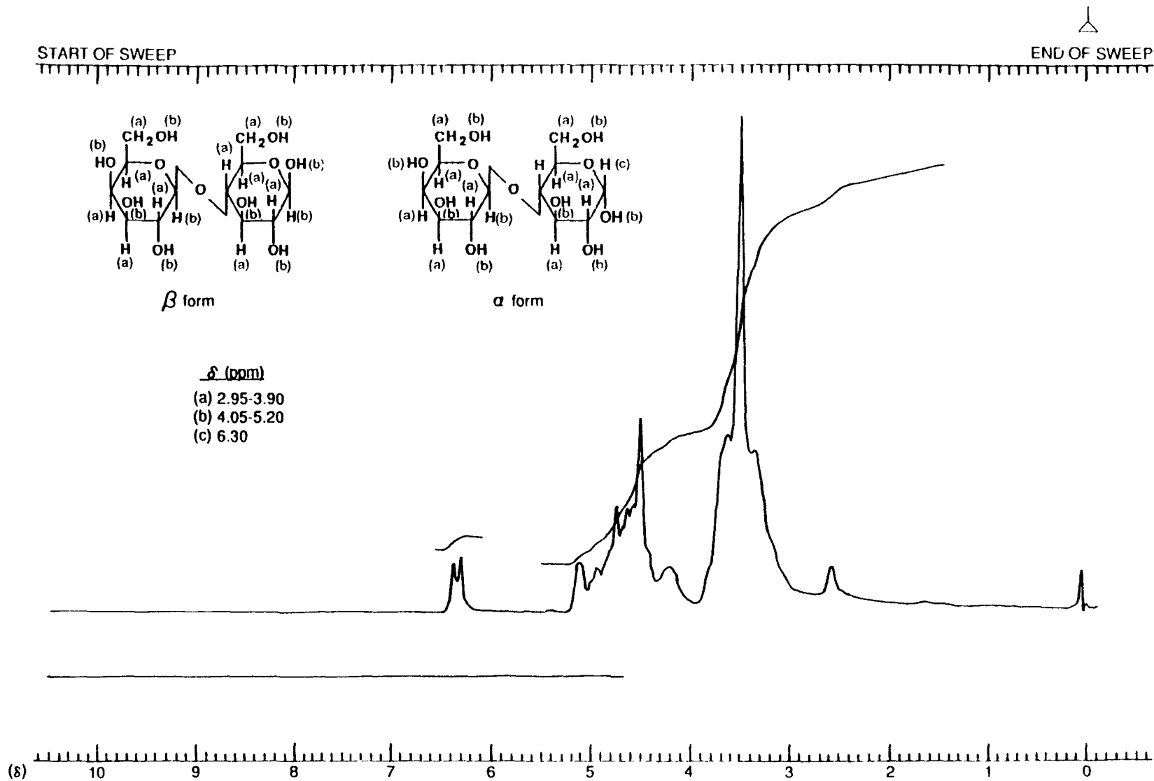
FIGURE 5. NUCLEAR MAGNETIC RESONANCE SPECTRUM OF LACTOSE
