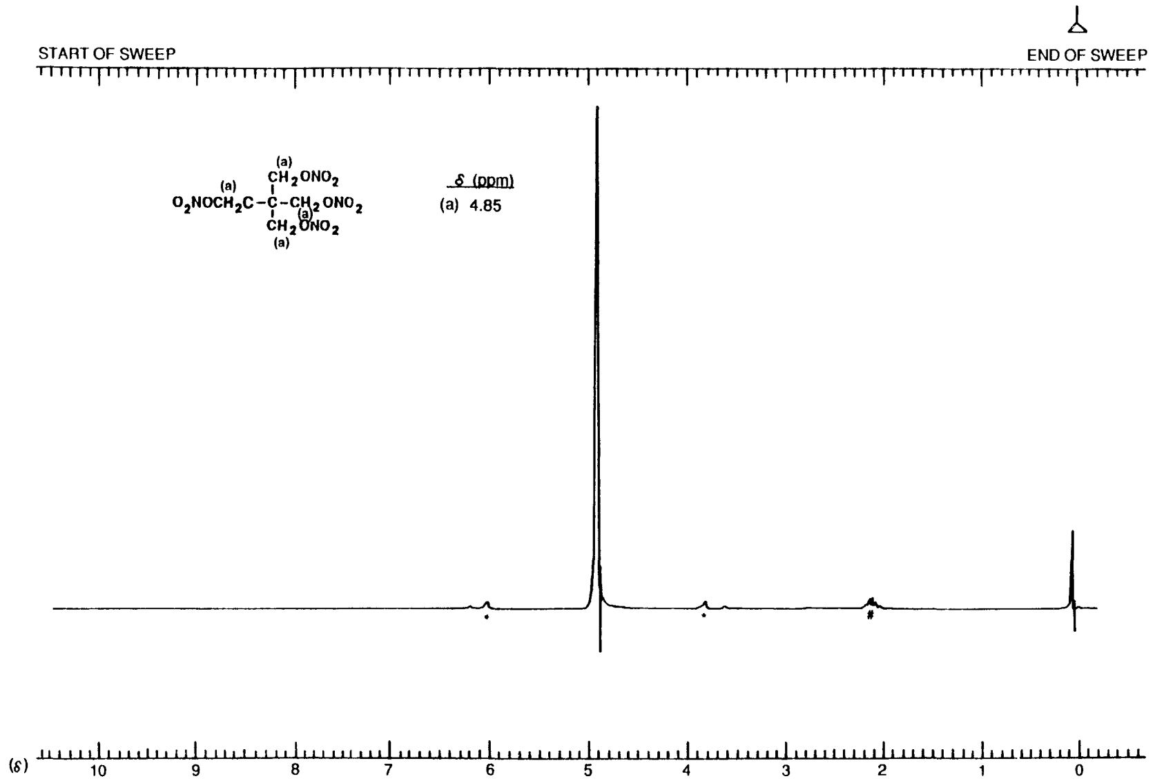
FIGURE 4. NUCLEAR MAGNETIC RESONANCE SPECTRUM OF A PETN ACETONE EXTRACT OF PETN, NF (LOT NO. G23-H2) IN ACETONE-d 6
