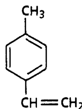
para-Vinyl Toluene (32%-35%)
