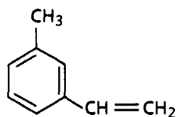
meta-Vinyl Toluene (65%-71%)
