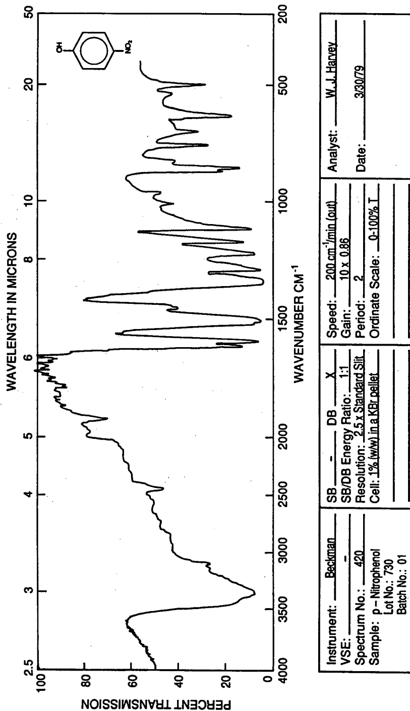
FIGURE E1 Infrared Absorption Spectrum of p-Nitrophenol
