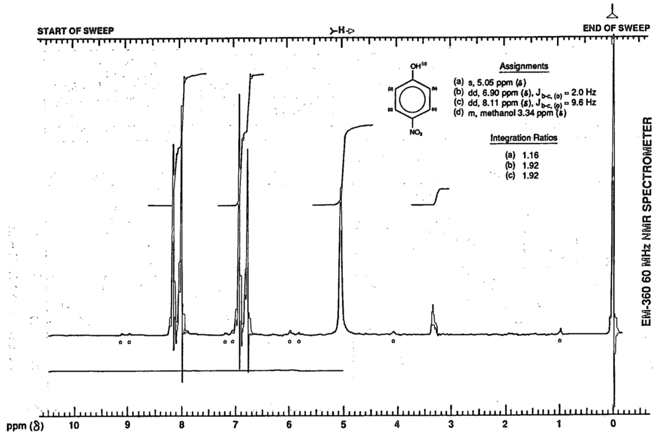
FIGURE E2 Nuclear Magnetic Resonance Spectrum of p -Nitrophenol
