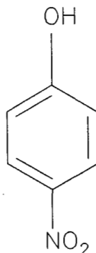
p -NITROPHENOL
