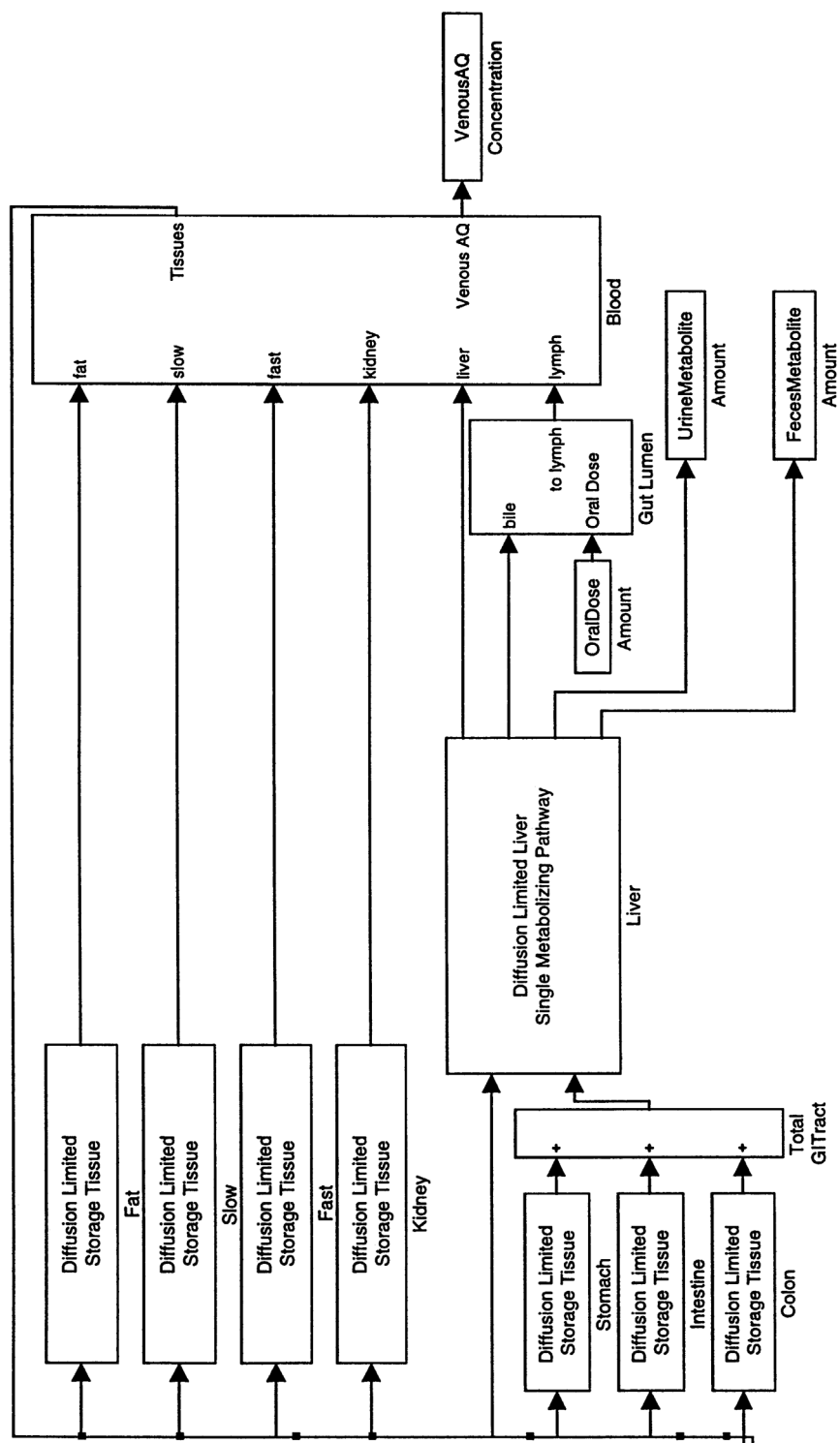
FIGURE 6 Schematic Representation of the Physiologically Based Pharmacokinetic Model for Anthraquinone
